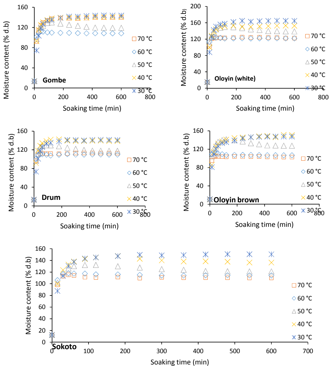
Fig. 1. Moisture content vs soaking time at different temperature Table 4. Model parameter for modelling of Gombe variety
