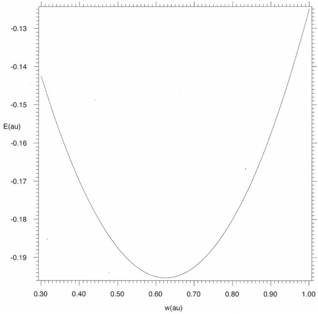
Fig. 1. E_+ - mc^2 versus w for the lowest positive-energy state of Ps in the Hartree model
