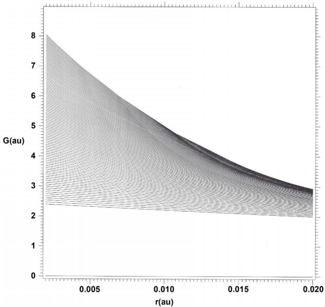
Fig. 5. G_{-1}(r) versus r in the negative-energy region of the spectrum for the sweep of w values used in the calculation.
