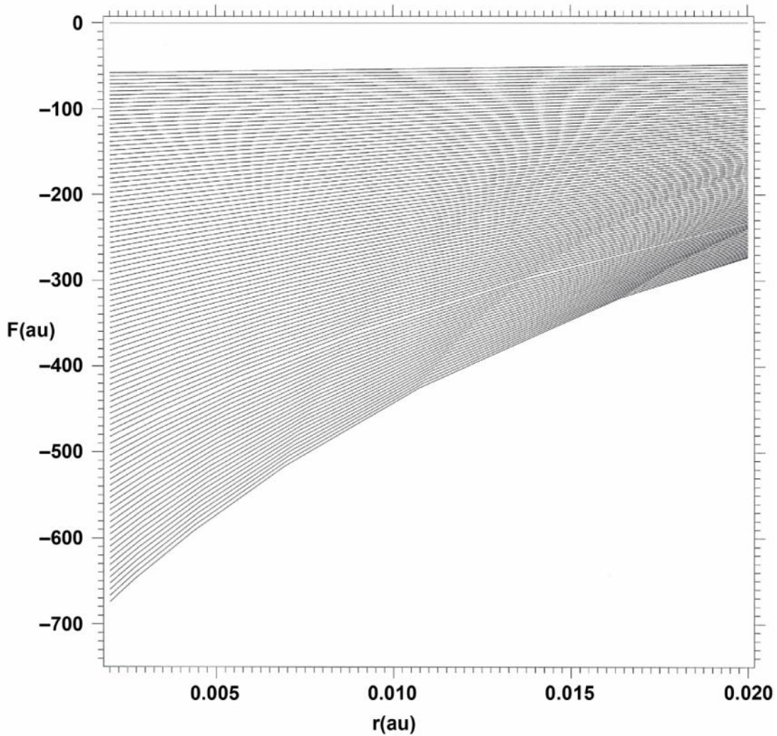
Fig. 6. F_{-1}(r) versus r in the negative-energy region of the spectrum for the sweep of w values used in the calculation.
