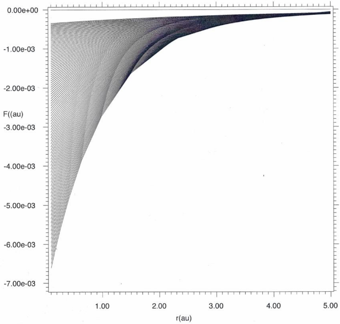
Fig. 3. F_{-1}(r) versus r in the positive-energy region of the spectrum for the sweep of w values used in the calculation
