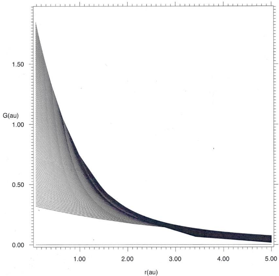
Fig. 2. G_{-1}(r) versus r in the positive-energy region of the spectrum for the sweep of w values used in the calculation
