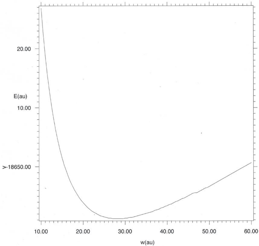
Fig. 4. E_- versus w for the lowest negative-energy bound state for Ps in the Hartree model.
