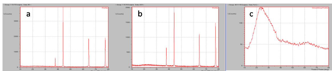
Fig. 1. XRD pattern of Fe NP a. SHB 13 b. SHB 204 c. surfactin
