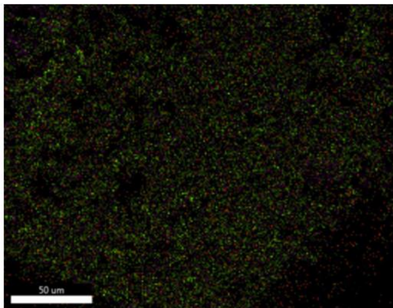
Fig. 10. Elemental map of (●) Oxygen (●) Copper
