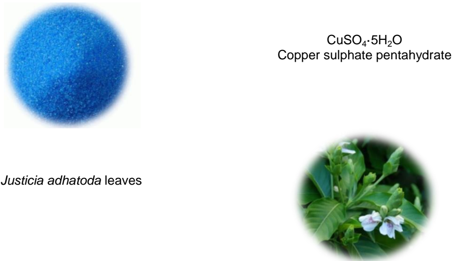
Fig. 1. Chemicals used
