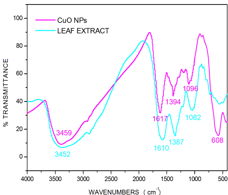
Fig. 5. FTIR spectra of CuO NPs and Justicia Adhatoda leaf extract
