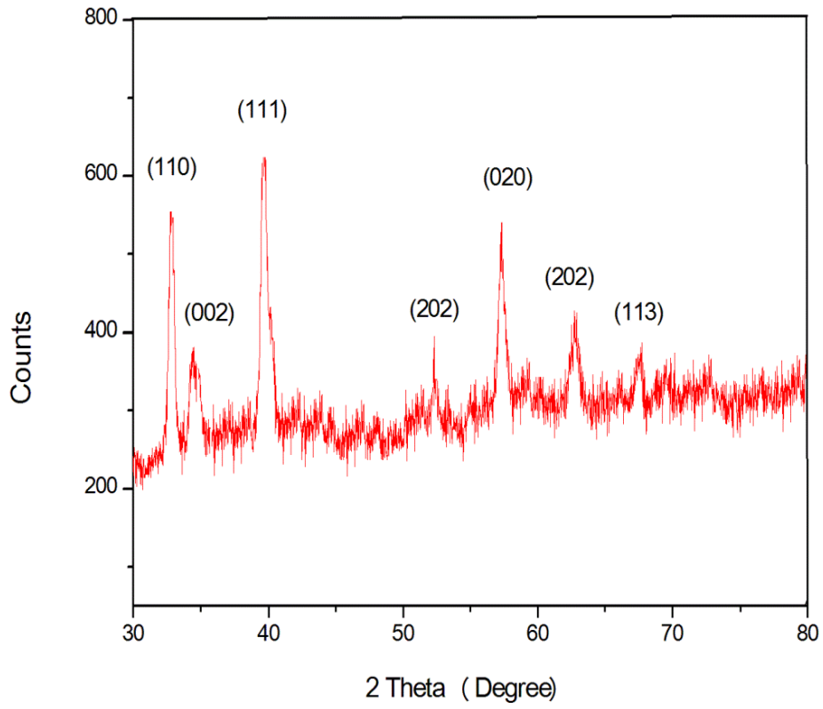
Fig. 6. XRD pattern of CuO NPs
