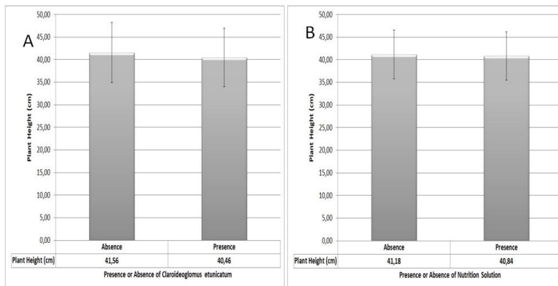
Fig. 2. Relationship between the presence and absence of claroideoglomus etunicatum (A) and nutritive solution (B) for the growth of salicornia ramosissima
