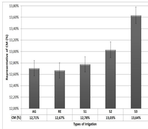
Fig. 1. Effect of saline irrigation (AG - water); RE (Reject); S1 (Reject + 1 NaCl); S2 (Reject + 2 NaCl) and S3 (Reject + 3NaCl) on the mycorrhizal colonization (MC) of salicornia ramosissima
