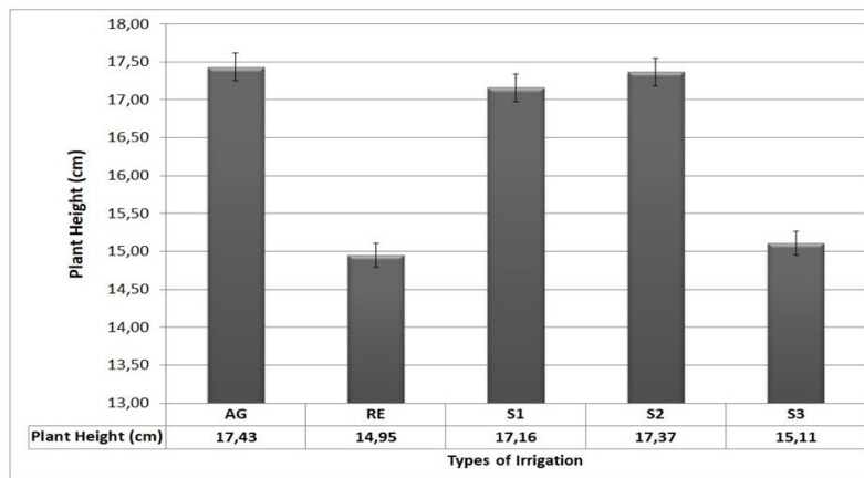
Fig. 3. Height of salicornia ramosissima irrigated with AG (water), RE (Reject), S1 (Reject + 1NaCl), S2 (Reject + 2 NaCl) and S3 (Reject + 3 NaCl)
