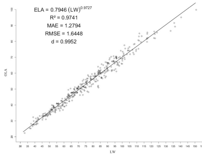
Fig. 3. Equation of power model, determination coefficient ( R^2 ), the mean absolute error (MAE), the root mean square error (RMSE) and index d, using the foliar area observed (OLA) as dependent variable, in function of the product of the length and width (LW) of leaflets of Acacia mangium Willd
