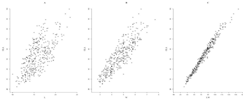
Fig. 2. Scatter plot of the actual leaf area in relation to length (L) (A), width (W) (B) and product of length with width (LW) (C)
