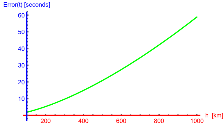
Fig. 2. Graph of the estimated error in the falling time, given by Eq. (33), versus the height h in the range h \in [100, 1000] [km]
