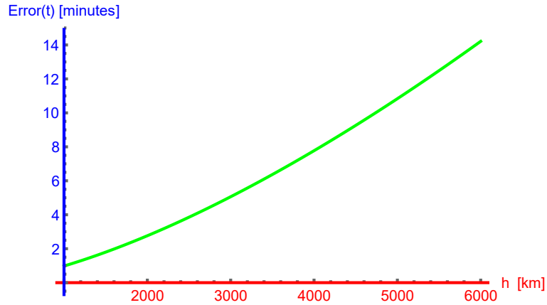
Fig. 3. Graph of the estimated error in the falling time, given by Eq. (33), versus the height h in the range h \in [1000, 6000] [km]
