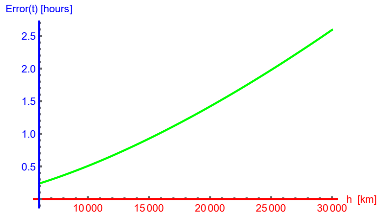
Fig. 4. Graph of the estimated error in the falling time, given by Eq. (33), versus the height h in the range h \in [6000, 30000] [km]
