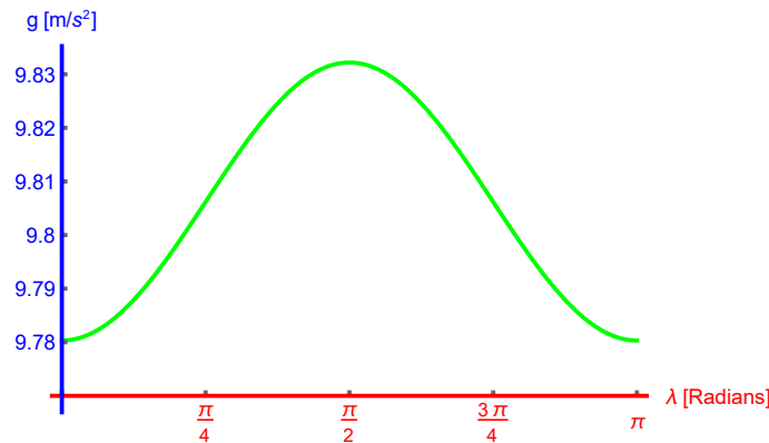
Fig. 1. Variation of the acceleration due to gravity of Earth g versus the latitude \lambda
